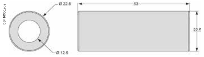
Brass
