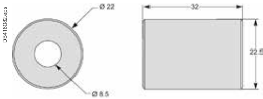
Brass
