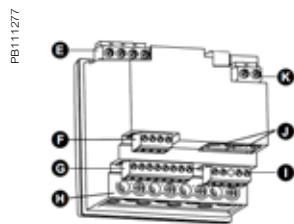
PM5000
